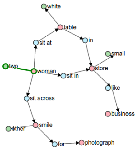
Fig. 2. A typical example of a scene graph (right) parsed from a set of reference image captions (left)
