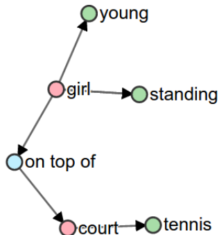
Fig. 1. Illustrates our method’s main principle which uses semantic propositional content to assess the quality of image captions. Reference and candidate captions are mapped through dependency parse trees (top) to semantic scene graphs (right)—encoding the objects (red), attributes (green), and relations (blue) present. Caption quality is determined using an F-score calculated over tuples in the candidate and reference scene graphs
